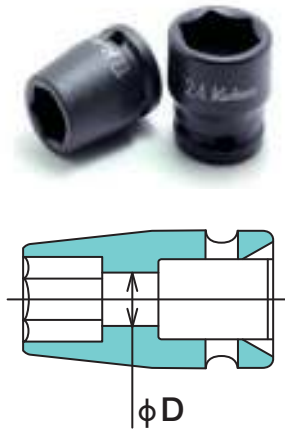
Standard Socket
