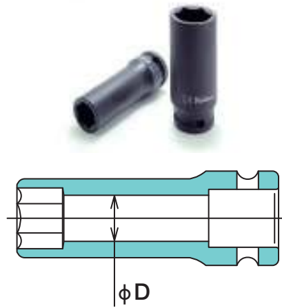
Deep Socket
